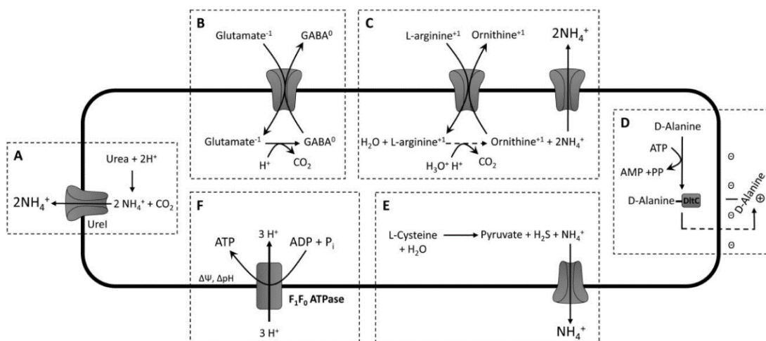
Fig. 2.4. Overview of metabolic pathways of genes assessed in this study. A. The urease gene converts urea to ammonia and CO 2 . Ammonia is exported from the cytoplasm using the UreI transporter, thus buffering the cell from its surrounding environment. B. Glutamate is imported into the cell by an antiport system and converted to GABA using the glutamate decarboxylase pathway while generating a \Delta\Psi and \Delta\text{pH} . H + consumption raises the intracellular pH. Adapted from Su and colleagues (2011) and Price and colleagues (2012). C. L-arginine is imported using an L-arginine–ornithine antiporter and converted into citrulline and ammonia by the arginine deiminase enzyme. Citrulline is further catalysed to ornithine and ammonia, while consuming H + . Ammonia is exported from the cytoplasm potentially using the UreI transporter. D. D-Alanine is coupled to a DltC carrier protein, exported across the cytoplasmic cell membrane and used for esterification of teichoic acids associated with the cell wall. This esterification results in a positive charge of the cell wall. Adapted and simplified from Peschel and colleagues (1999). E. Cysteine is converted to ammonia, hydrogen sulfide and pyruvate by the cystathionine \gamma -lyase. Ammonia is exported from the cytoplasm using the potentially via the UreI transporter, thus buffering the cell from its surrounding environment. F. F 1 -F 0 -
