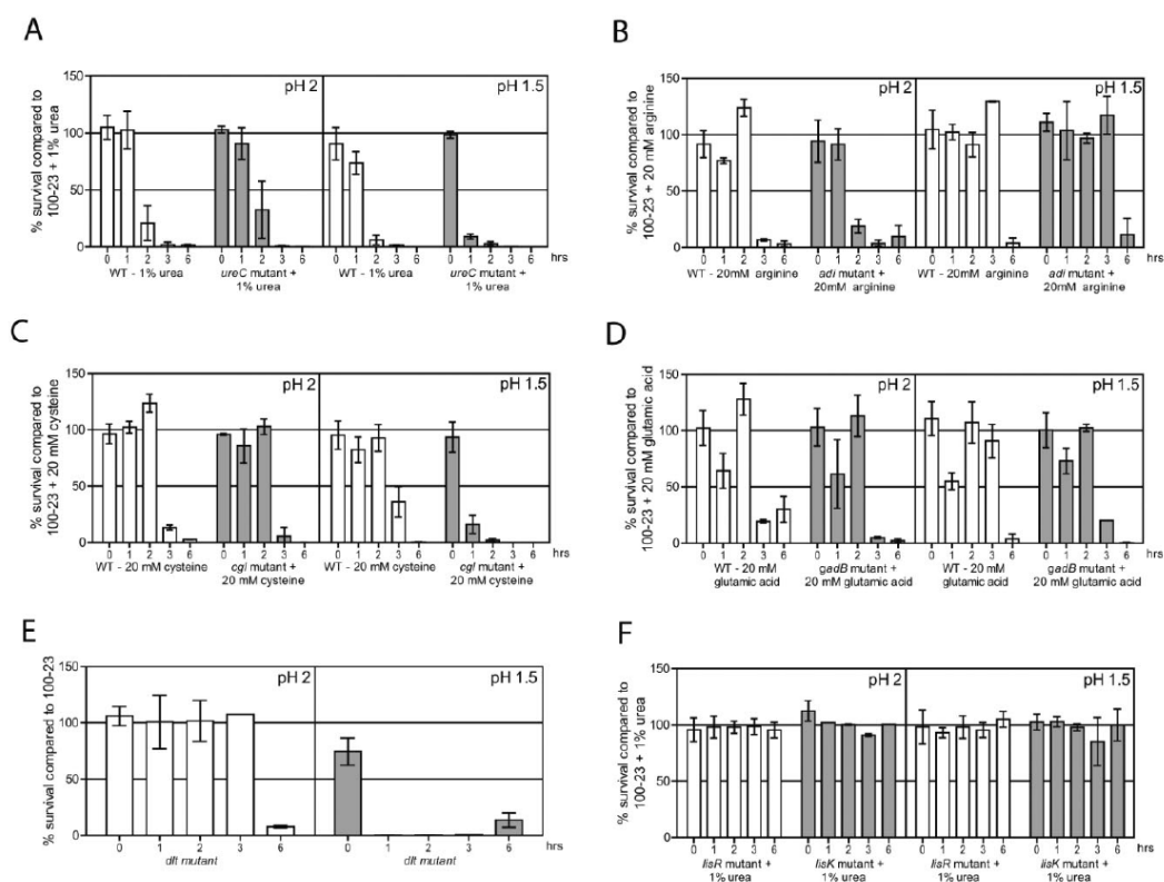
Fig. 2.1. Determination of the capacity of genes (Table 2.1) to confer survival under acidic conditions. The viability of strains was determined after incubation in artificial gastric fluid at pH 2 and 1.5 for 6 h at 37°C. Survival of (I) wild-type strains incubated without the substrate of the respective enzyme and (II) mutant strains incubated with the respective substrate are shown relative (%) to that of the wild-type strain incubated with the respective substrate. (A) ureC ; (B) adi ; (C) cgl ; (D) gadB ; (E) dltA ; and (F) lisR and lisK . Because there is no added substrate for the dltA , lisR and lisK genes, only the survival of the mutants was compared with the wild-type. Data are shown as means with standard deviations of triplicate independent experiments (biological replicates).
