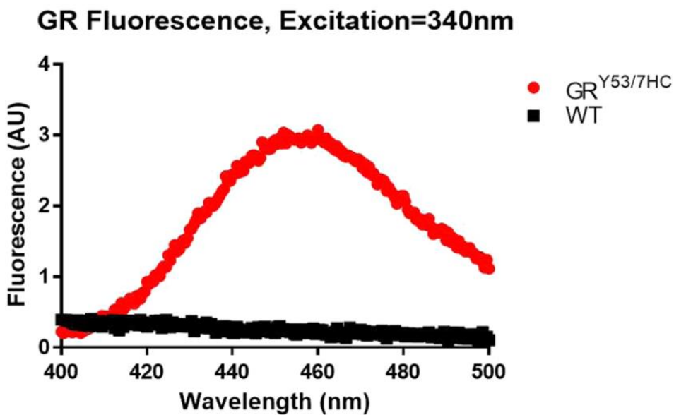
Figure 6. Fluorescence scans using an excitation wavelength of 340 nm confirms the presence of 7HC ( \lambda_{max} = 455 nm) in the GR Y53/7HC mutant (red), but not in a similar purification of wild-type GR (black). The concentration of wild-type GR is 4-fold more than that of GR Y53/7HC .
